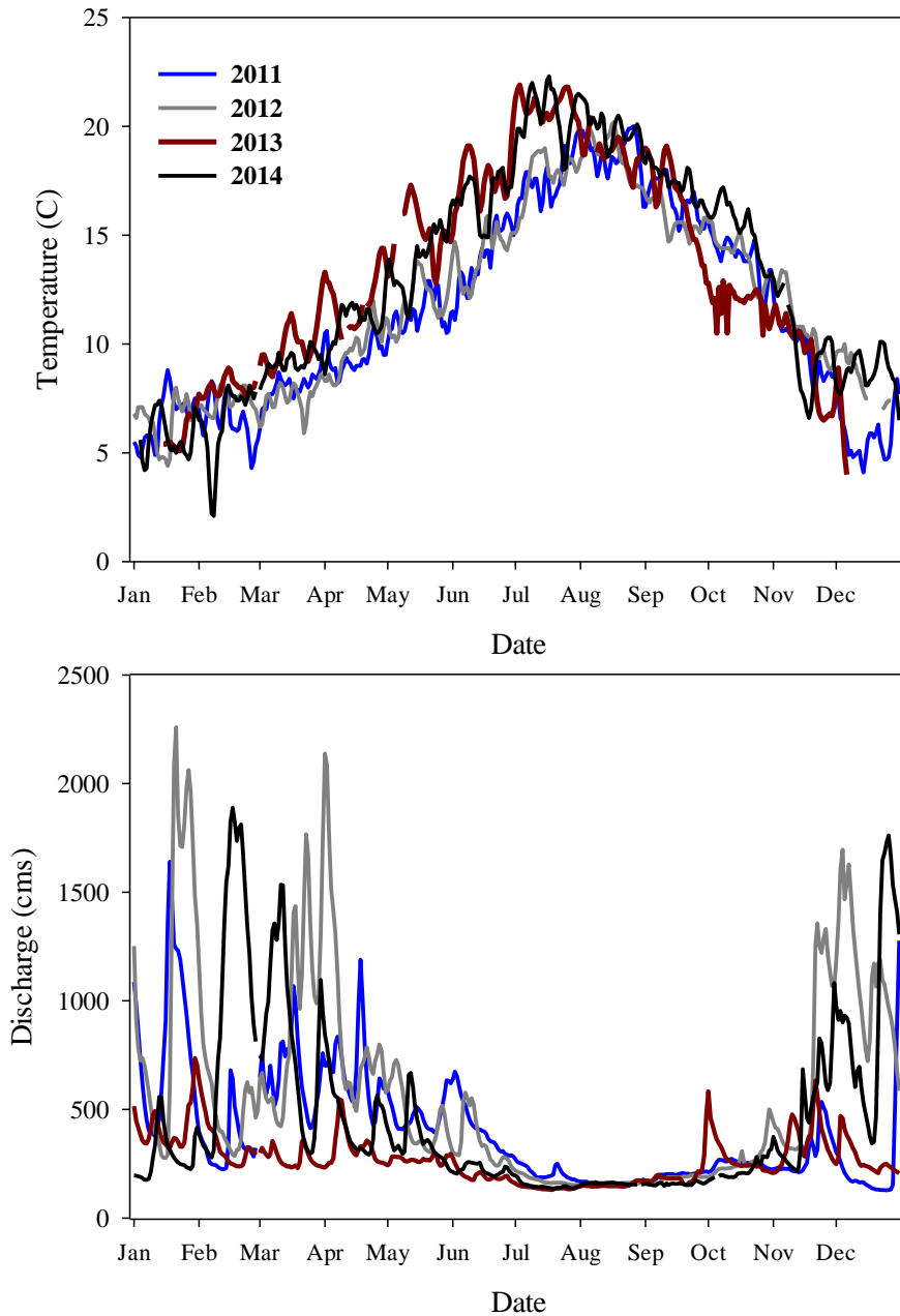
Figure 4. Mean daily Willamette River water temperature ( ^{\circ}\text{C} , top panel) and mean daily Willamette River discharge (cms) recorded at the USGS gauge at Albany, OR, in 2011-2014 (bottom panel). Data were collected from http://ida.water.usgs.gov/ .
