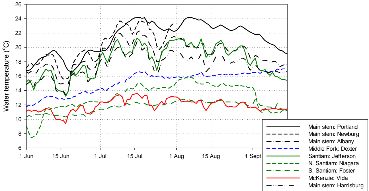
Figure 5. Mean daily water temperatures (°C) recorded at USGS gauge sites in the main stem Willamette, Middle Fork Willamette, Santiam, and McKenzie rivers during the spring Chinook salmon migration in 2014.
